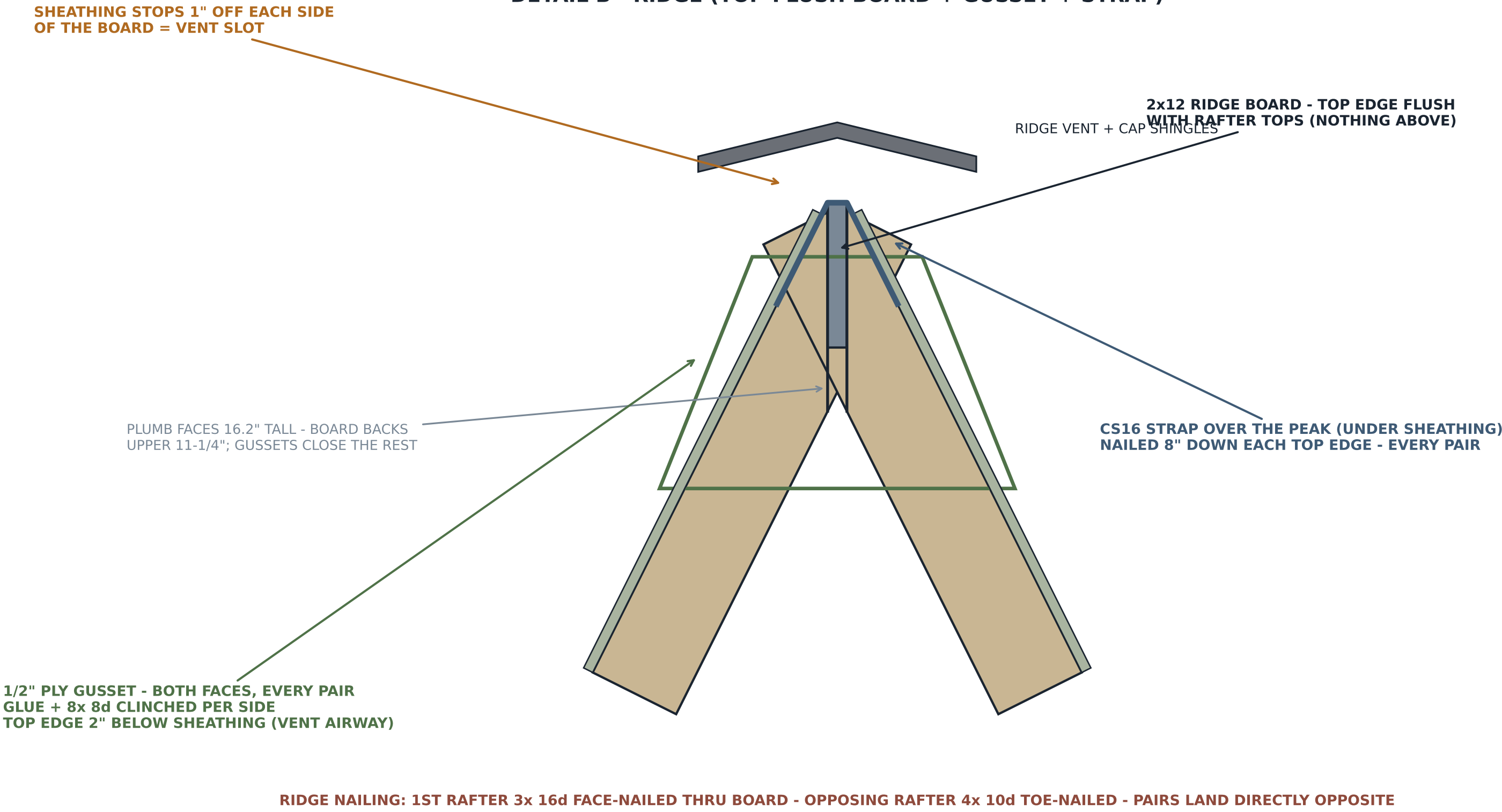
DETAIL B - RIDGE (TOP-FLUSH BOARD + GUSSET + STRAP)
