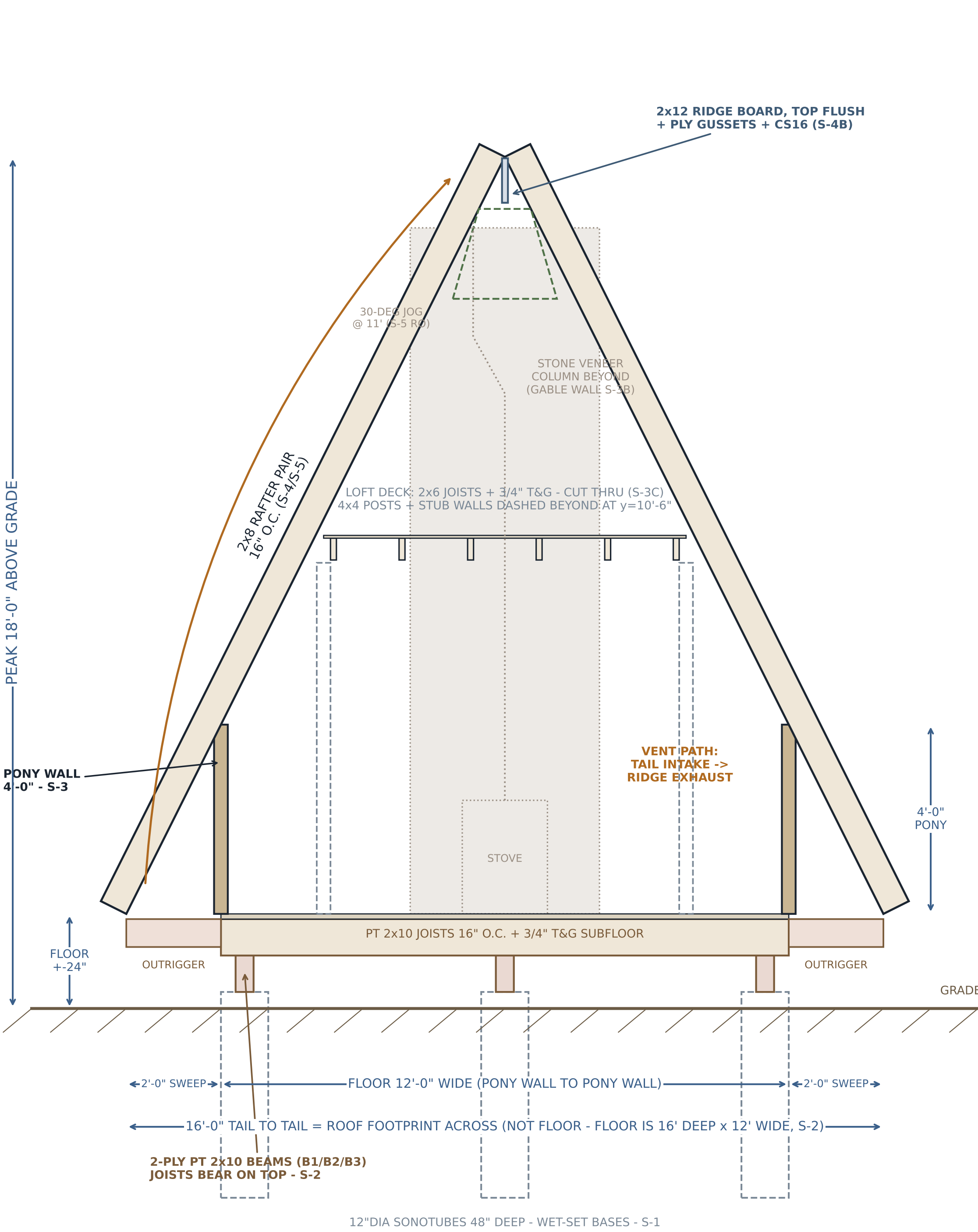
SECTION A-A - CUT AT y=11'-6" LOOKING TOWARD STOVE END
