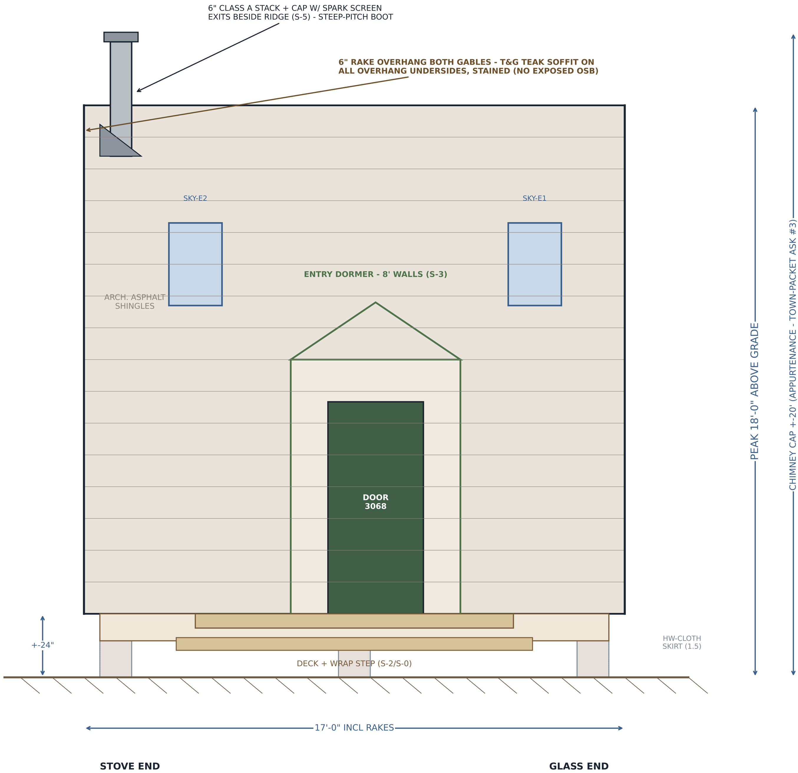
SIDE ELEVATION - ENTRY SIDE, VIEWED FROM OUTSIDE (STOVE LEFT / GLASS RIGHT - THE NEIGHBOR VIEW)
